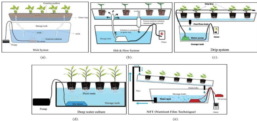
Fig 3. Diagram of Various Structures of Hydroponic System
